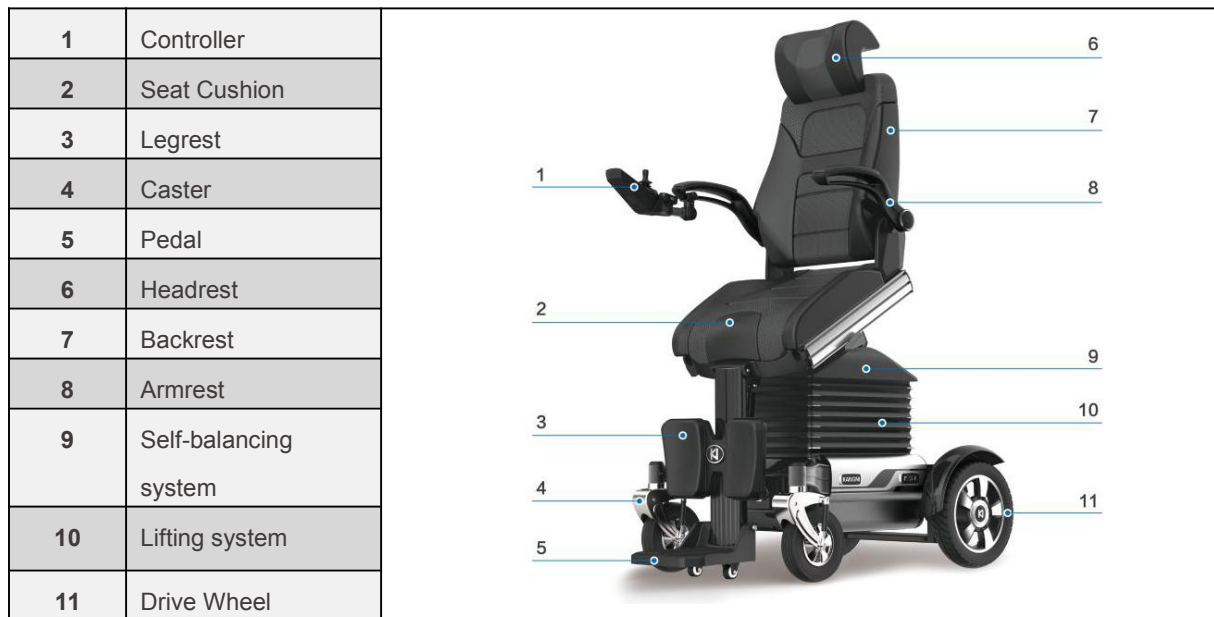
Main components of the electric wheelchair
